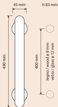
Maniglione. Interassi disponibili 300-400-500-600-800. / Pull handle. Available distances 300-400-500-600-800.
