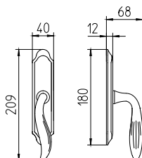
982/M cremonese window lever handle
