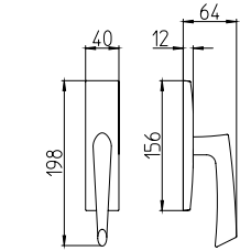
352/M cremonese window lever handle
