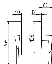
1692/M cremonese window lever handle
